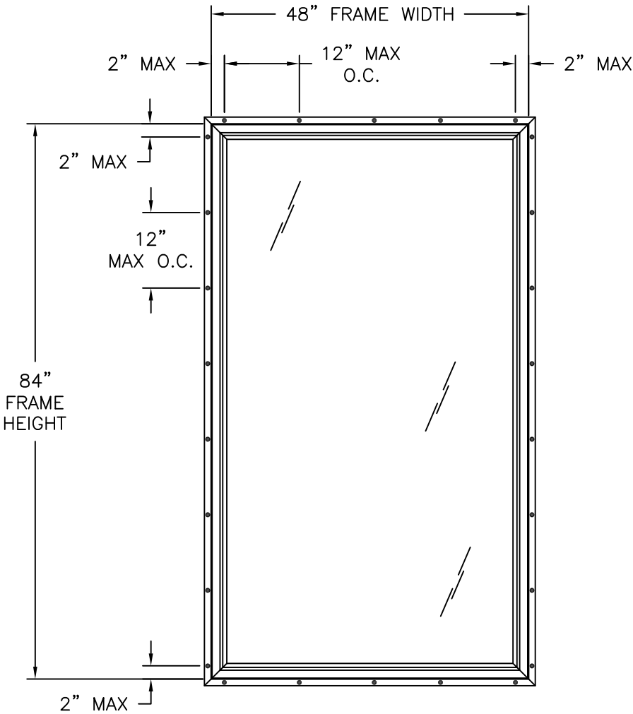
200/275 VINYL PICTURE WINDOW EXTERIOR VIEW
