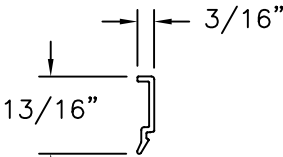
GLAZING BEAD (1703-R) EXTRUDED RIGID PVC
